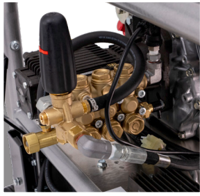
Direct Drive EZ4040 Pump
